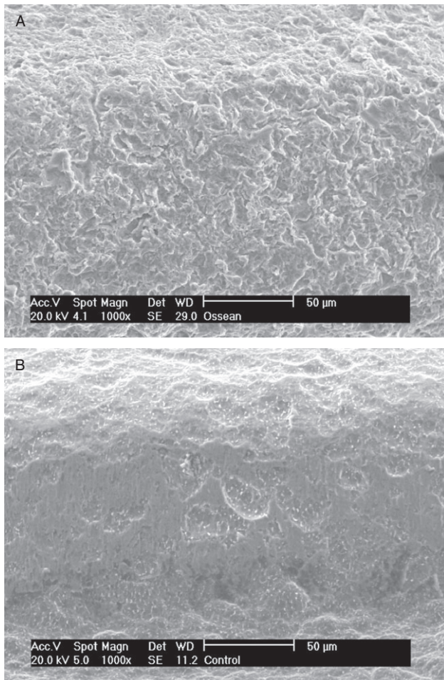
Figure 1 Scanning electron microphotograph of the implant surface topographies evaluated A, Ossean® and B, dual acid-etched surface.
