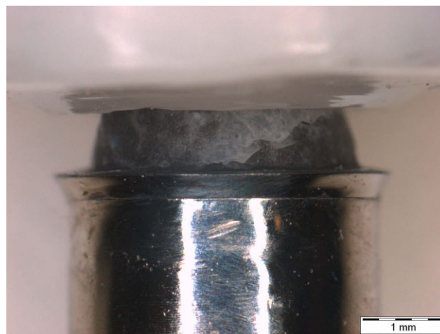
Figure 3 Failure mode of all tested specimens were completely adhesive, leaving the detached zirconia coping and titanium insert undamaged.
