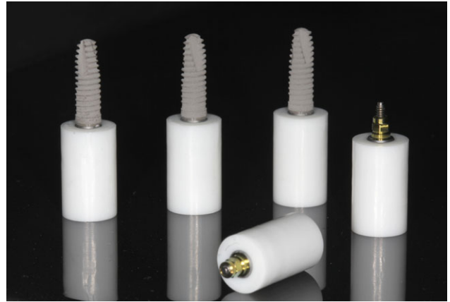
Figure 1 Test specimens: two-piece zirconia abutments connected to internally hexed implants. Zirconia copings were modified for the test setup.
