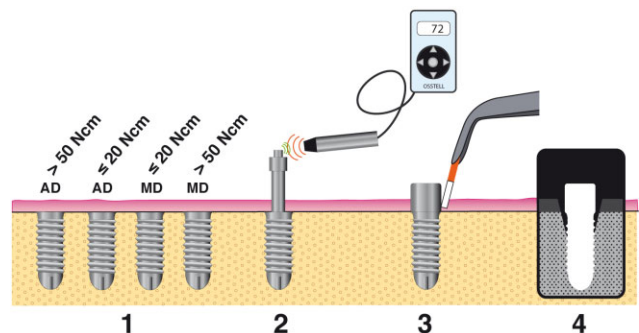
Figure 2 Schematic illustration of the study protocol: (1) implant placement with different insertion torques (≤20 Ncm, >50 Ncm) and different implant neck designs (AD: anodized design, MD: machined design), (2) implant stability measurements by resonance frequency analysis using Osstell® mentor and Smartpeg™ abutments, (3) collection of crevicular fluid for detection of interleukin-1 \beta , (4) radiographic assessment of peri-implant bone level.
