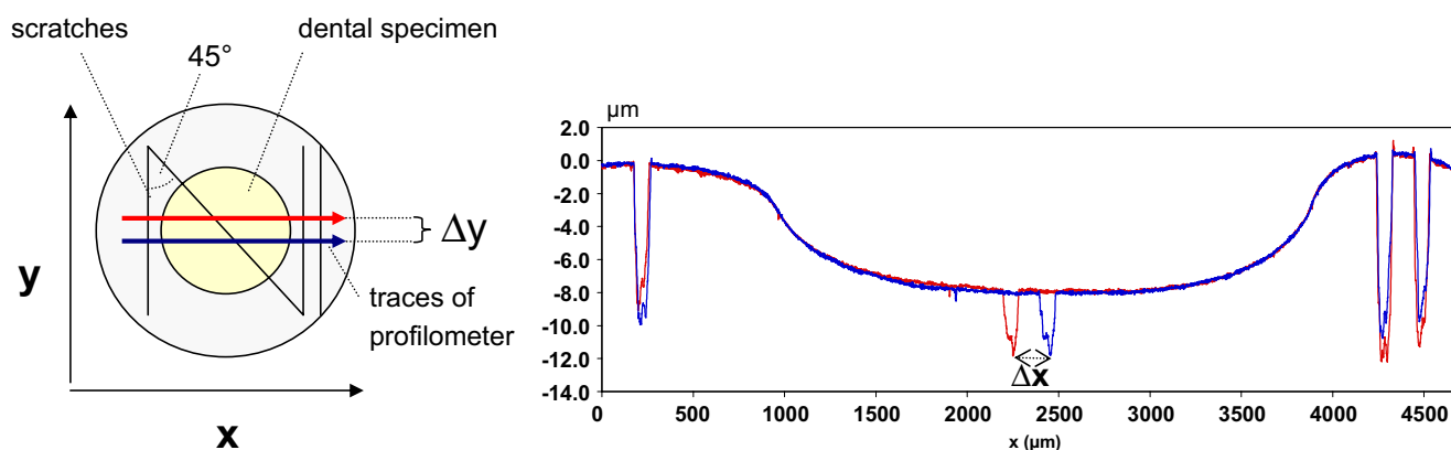
Fig. 1 Left Schematic drawing of a specimen with intentionally placed scratches used to determine reproducibility of profilometric assessment. Right Exemplary surface profile gained from a specimen
