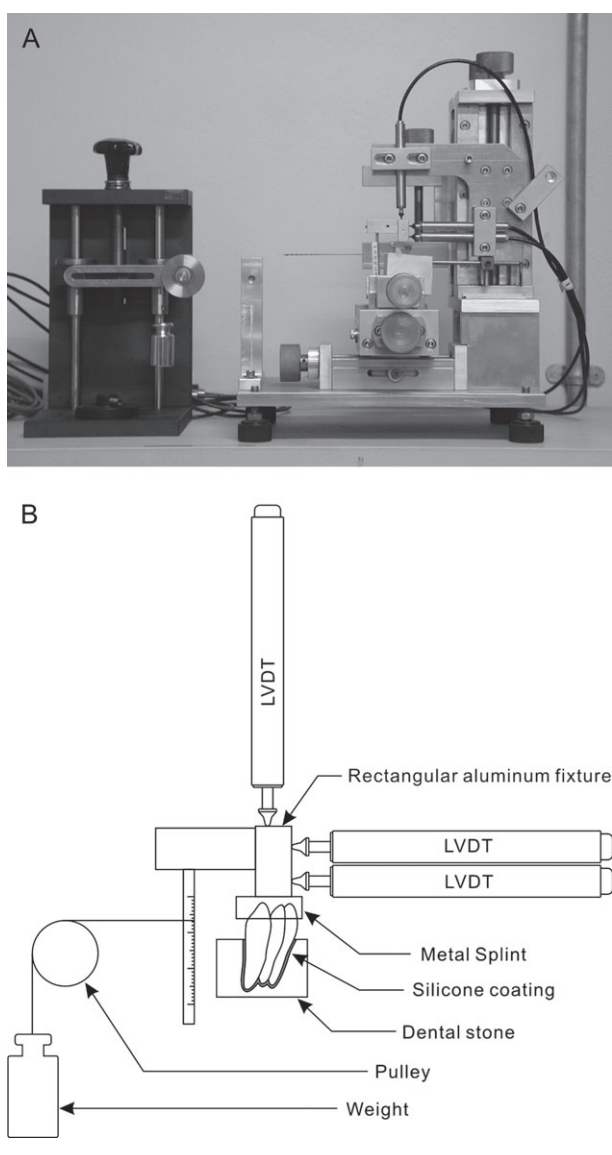
Figure 1 (A) Overall set-up of the apparatus. A pulley was used to apply a horizontal force while three linear variable differential transformers (LVDTs) were used to detect the displacement of the anterior segment. (B) Schematic drawing of the anterior segment, horizontal force, and LVDTs.
