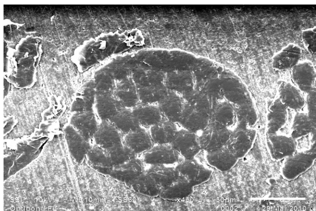
FIGURE 7. Scanning electron microscope micrograph of polyethylene fibers pre-impregnated with Optibond FL adhesive resin (section view, original magnification \times 450 ).
