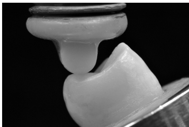
FIGURE 4. Specimen (onlay) positioned in testing machine at a 30-degree angle. Load is applied through single contact between composite resin cylinder and palatal cusp.
