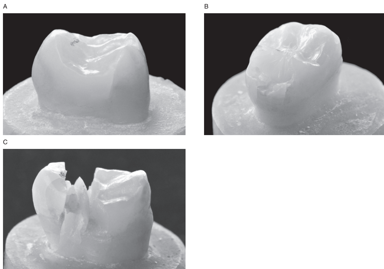
FIGURE 6. A, Onlay with fiber reinforcement that survived (total 180,000 cycles, no failure). B, Non-destructive fracture of inlay at 1,050 N. C, Catastrophic failure of onlay with fiber reinforcement at 750 N.
