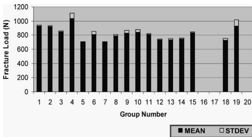
Figure 6 Mean preload values and standard deviations for each prosthetic screw group.
