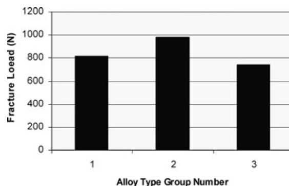
Figure 8 Mean fracture load values for the three screw groups classified by alloy type (composition). (Significant difference between fracture load values for the three groups at p < 0.001 ) 1 = Gold alloy screw from NB, 2 = Palladium alloy from NB, 3 = Gold alloy from SG.
