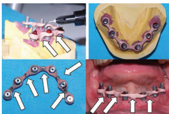
Figure 6 Attaching opaquet framework to titanium abutment cylinders (top left). Occlusal view of framework attached to titanium abutment cylinders (top right). Tissue view of framework with attached titanium abutment cylinders (bottom left). Intraoral view of try-in titanium abutment cylinder—framework complex seated on implants; also being used as a verification jig. (bottom right). Note tissue stops (arrows).
