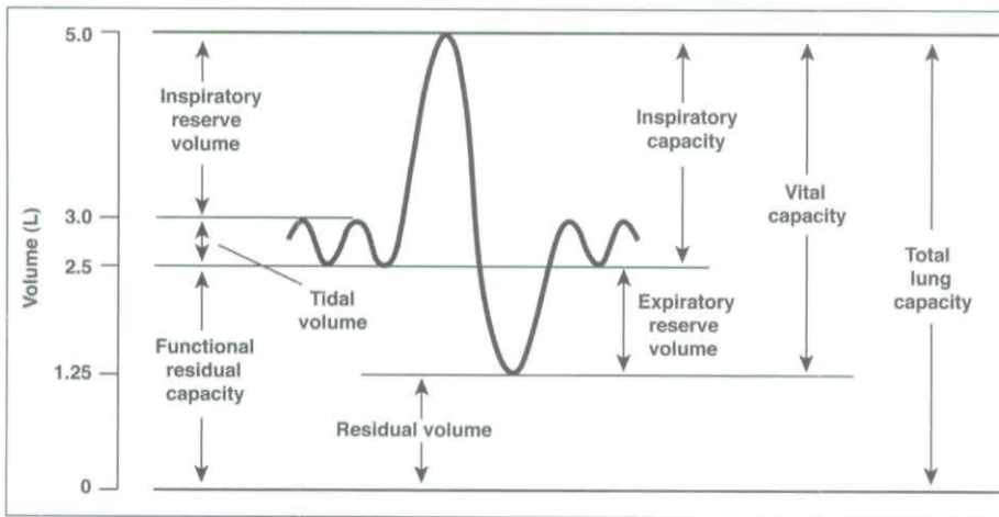
Figure 2. Dynamic lung volumes and capacities. Figure used by permission. 21
