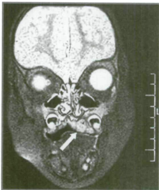
Figure 3. MRI showing three lobes
