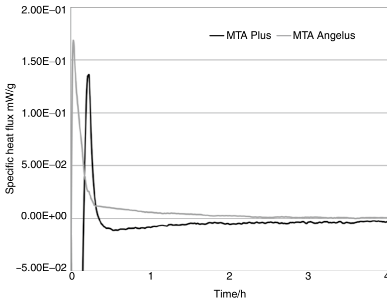
Fig. 2.4 Graphical representation of heat flux generated with time for MTA Plus and MTA Angelus
